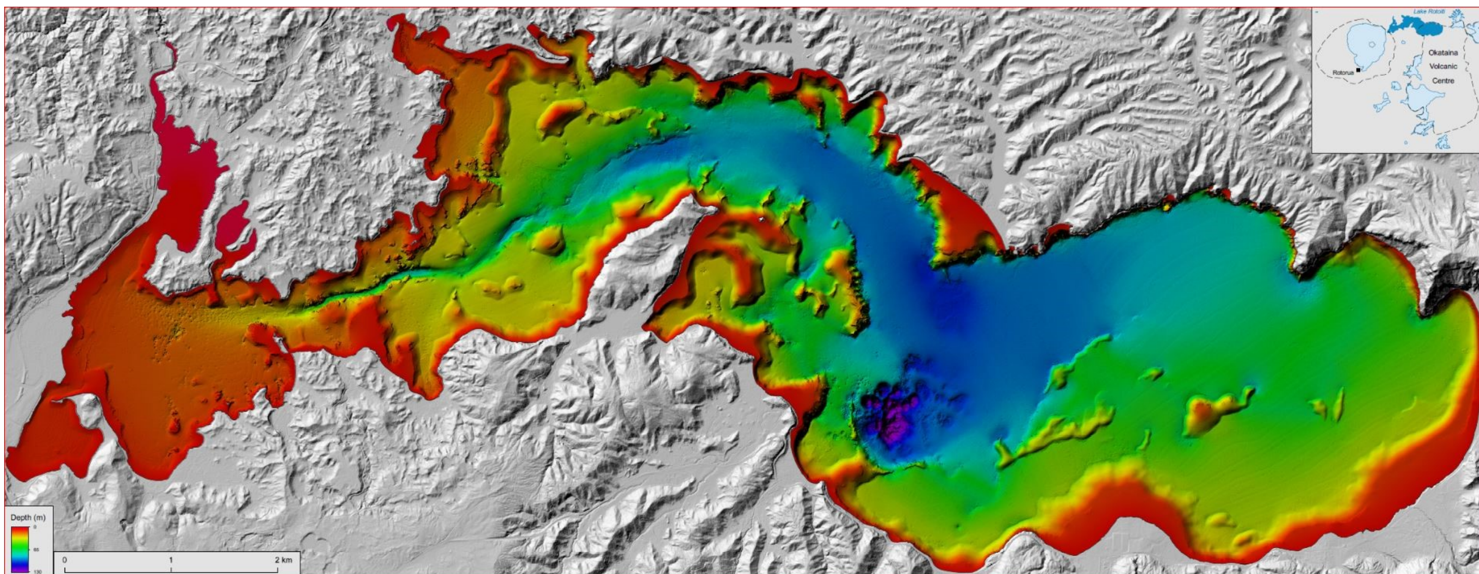
Lake Rotoiti Bathymetry map prepared by GNS Science.
